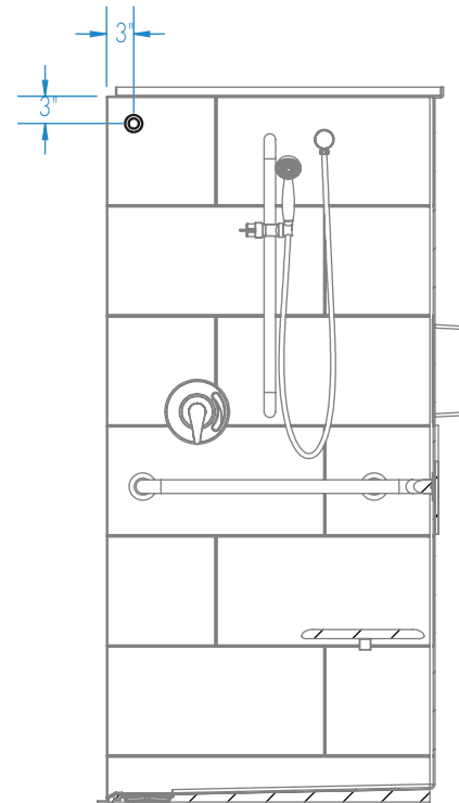
SECTION C-C
